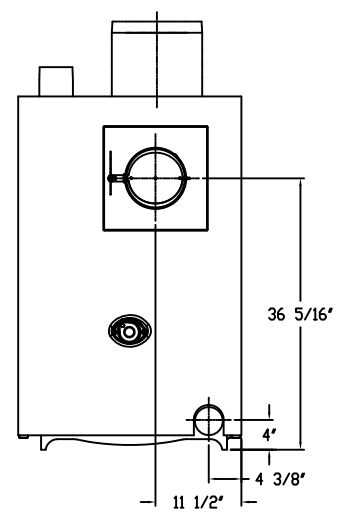
BACK
